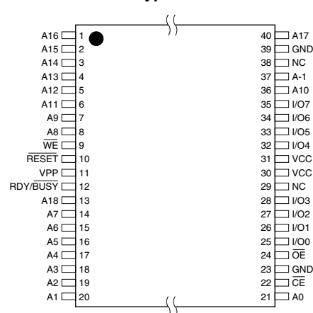
AT49BV008A(T) TSOP Top View Type 1
