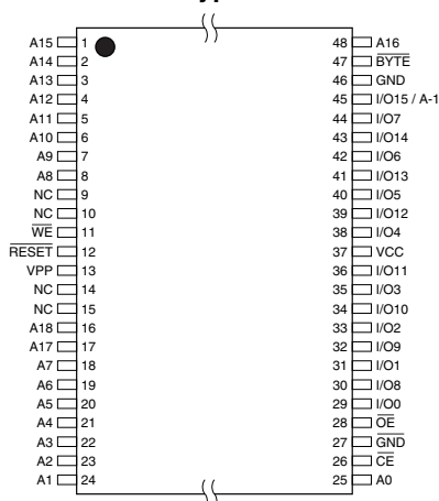
AT49BV8192A(T) TSOP Top View Type 1
